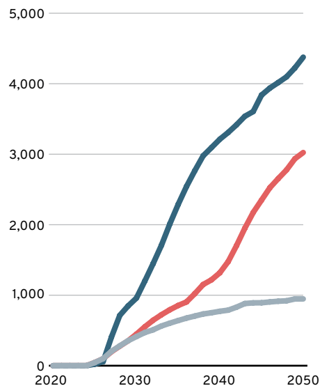
Electricity required for hydrogen production, in TWh/y
