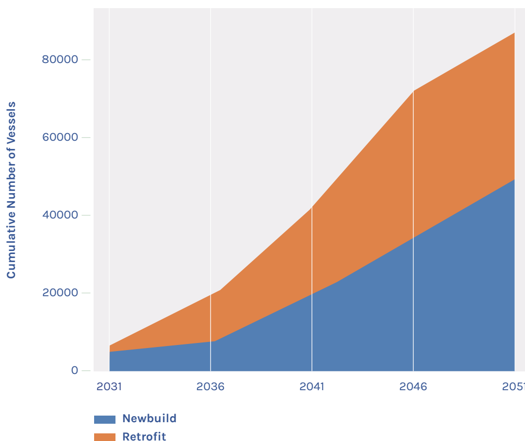
Figure 1: Similar magnitudes of newbuilding and retrofitting to SZEf use will be needed, unless ship lives are significantly reduced for the fossil fuelled fleet.
